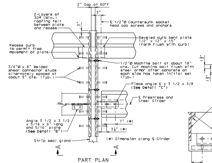
PART PLAN
