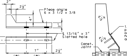
DETAIL "C"
