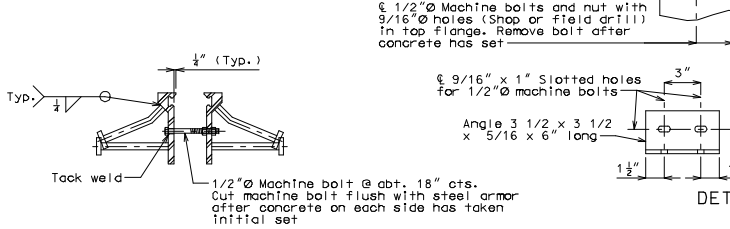
DETAIL "A"
