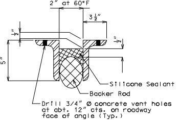
PART CROSS SECTION THRU EXPANSION JOINT
