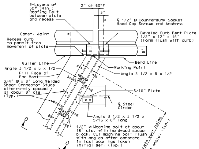
PART PLAN
