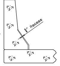
PART SECTION A-A
