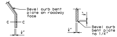
SECTION C-C
