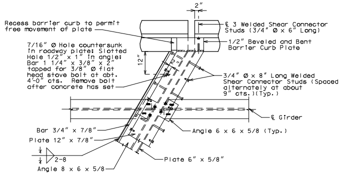
PART PLAN
