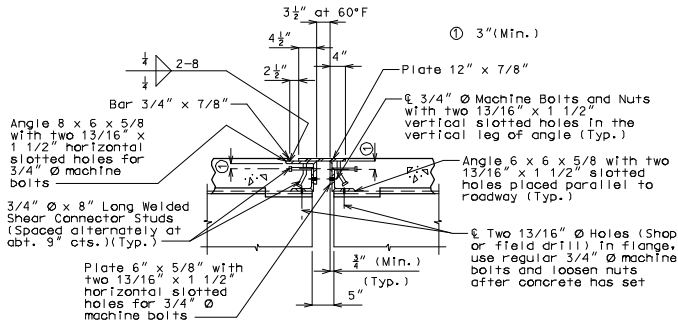
PART SECTION AT INTERMEDIATE BENT
