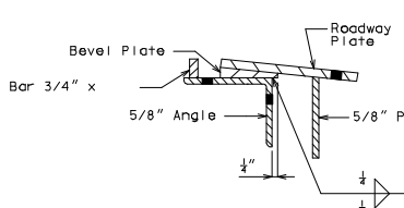
PART SECTION THRU BEVEL PLATE
