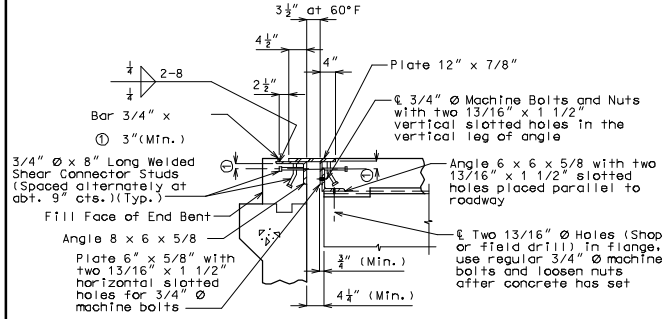
PART SECTION AT END BENT
