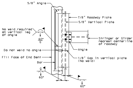
PERMISSIBLE FIELD SPLICE AT END BENT
