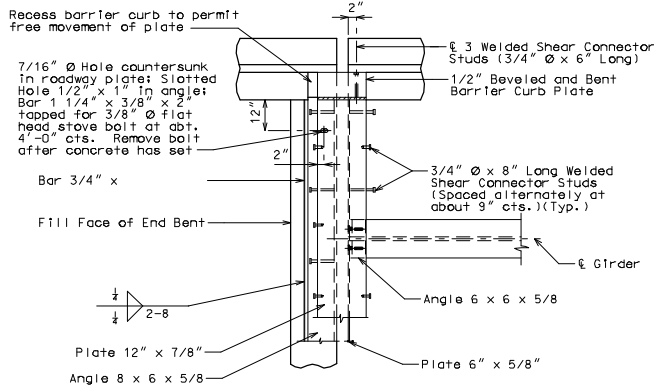
PART PLAN
