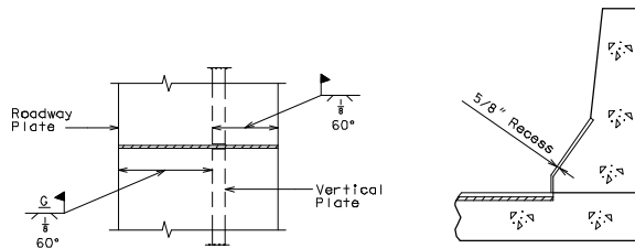
PART PLAN ROADWAY PLATE AND VERTICAL PLATE
