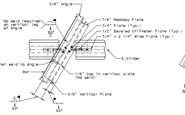
PERMISSIBLE FIELD SPLICE AT INT. BENT
