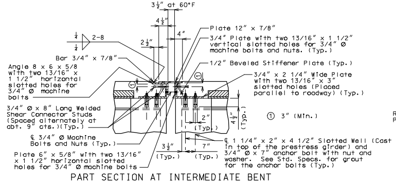
PART SECTION AT INTERMEDIATE BENT
