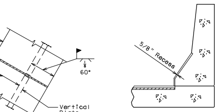
PART SECTION B-B
