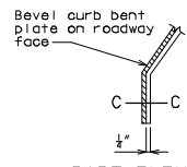
PART SECTION AT END OF BEVELED CURB BENT PLATE
