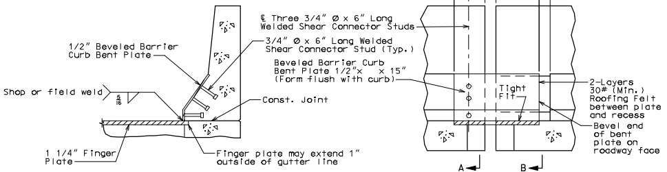
PART SECTION A-A
