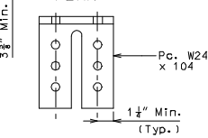
ELEVATION PC. W24 x 104
