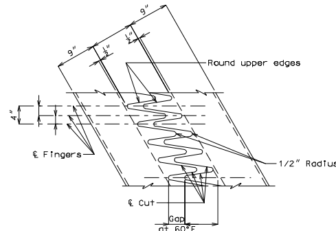
TYPICAL PLAN OF PLATE
