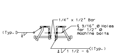
DETAIL "A"
