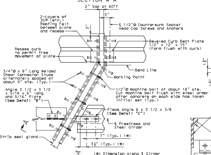
PART PLAN
