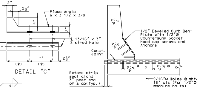
PART ELEVATION OF BARRIER CURB
