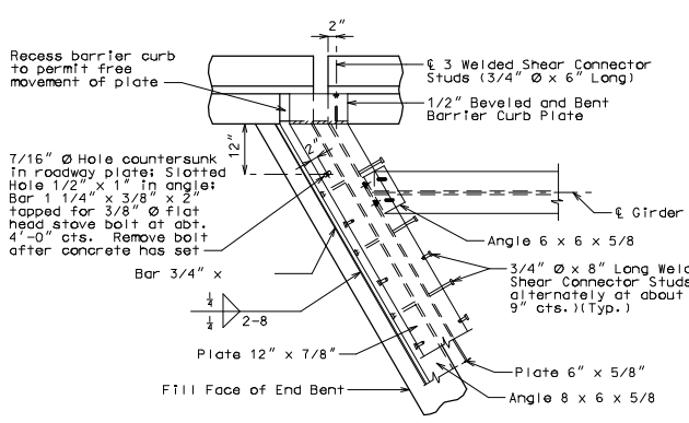
PART PLAN
