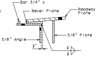
PART SECTION THRU BEVEL PLATE
