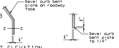
SECTION C-C
