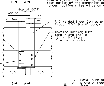
ELEVATION OF BARRIER CURB
