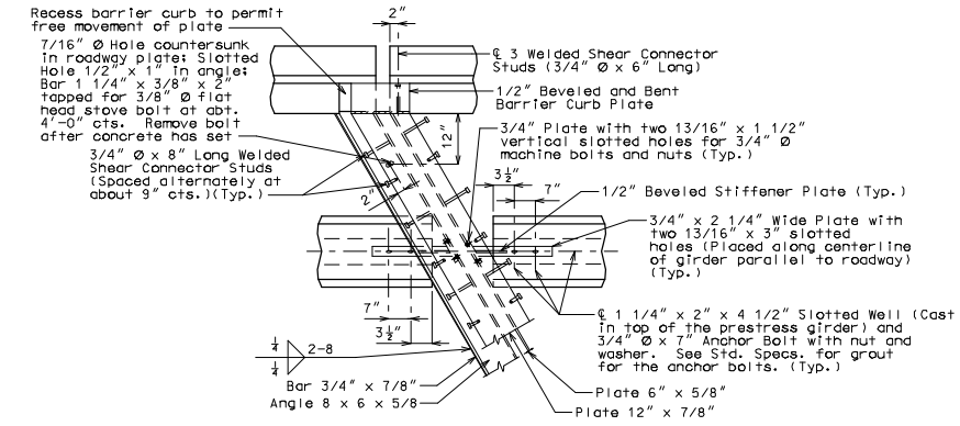
PART PLAN
