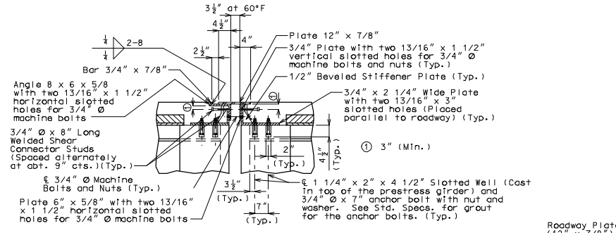
PART SECTION AT INTERMEDIATE BENT
