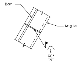
PART PLAN OF ANGLE AND BAR
