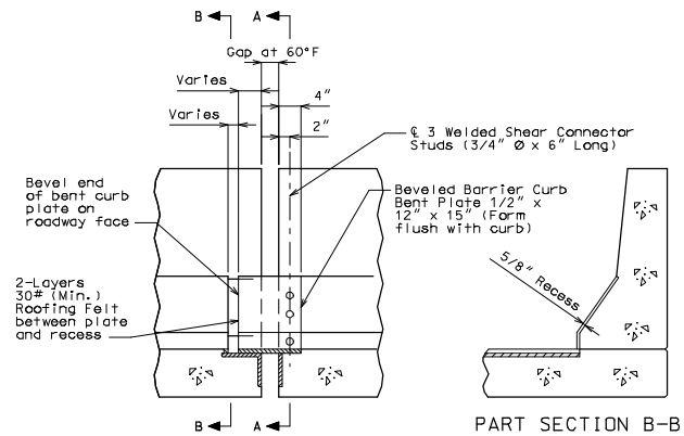
ELEVATION OF BARRIER CURB
