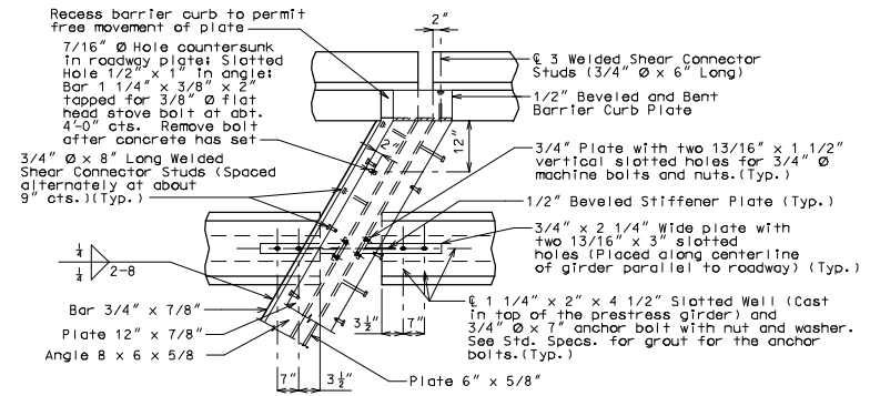
PART PLAN
