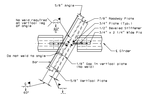
PERMISSIBLE FIELD SPLICE AT INT. BENT
