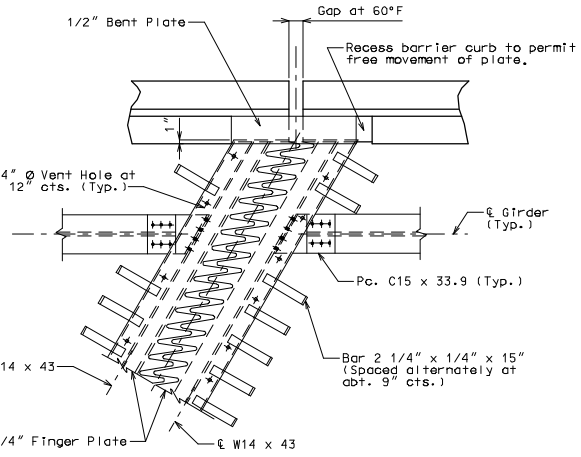
PART PLAN OF EXPANSION DEVICE
