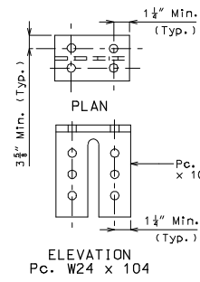
TYPICAL PLAN OF PLATE
