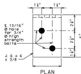
DETAIL OF FLANGE CONNECTION ANGLE
