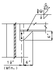
DETAIL "B"
