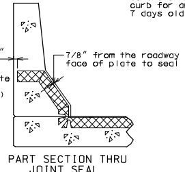
PART SECTION THRU JOINT SEAL
