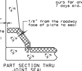
PART SECTION THRU JOINT SEAL
