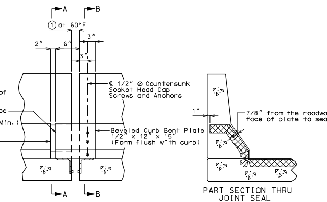
PART ELEVATION OF BARRIER CURB
