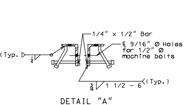
DETAIL "A"
