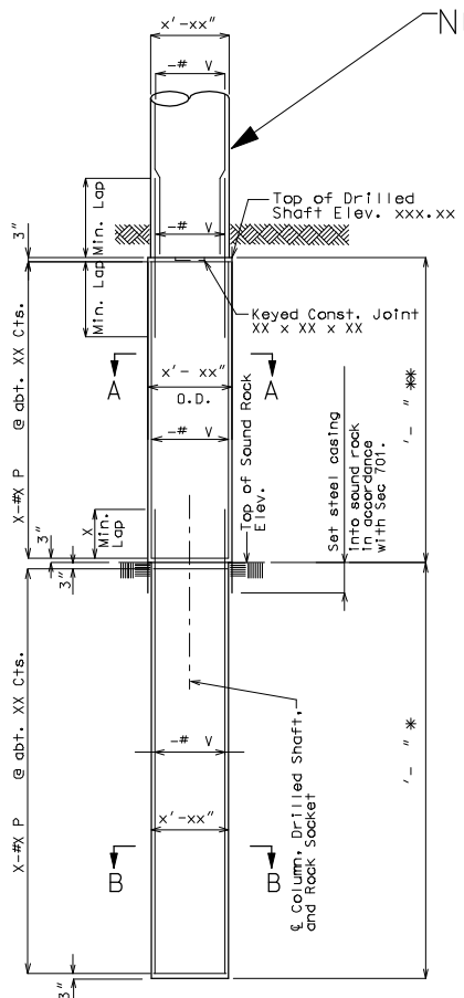
ELEVATION OF DRILLED SHAFTS AND ROCK SOCKETS
